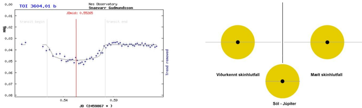
Myndir/Fig. 26a-b. a) Birtugildi TOI 3604 í þvergöngunni 14. október 2022. b) Niðurstöðurnar lýsa reikistjörnu með ~1% meiri geisla en uppgið gildi í veftóli TRESKA. – a) Results from October 14, 2022. Time is on the x-axis and magnitude on the y-axis. b) Geometry as a results of measurements. Images based on TRESKA website (Poddaný and others 2010).
