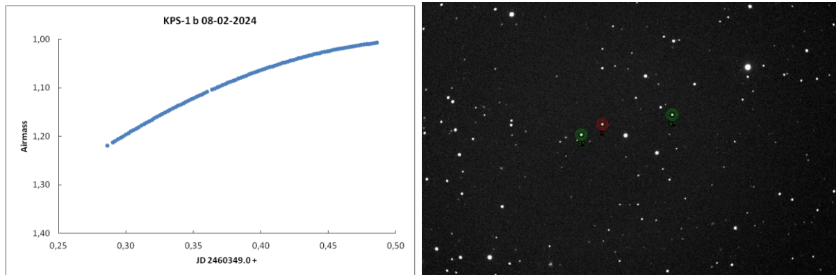
Myndir/Fig. 104a-b. a) Loftmassaferill KPS-1, 8. febrúar 2024. b) KPS-1 (í rauðum hring) og viðmiðsstjörnur (grænir hringir). – a) Airmass plots for KPS-1 on February 8, 2024. b) KPS-1 (red circle) and its comparison stars (green circles) used for magnitude estimations.
